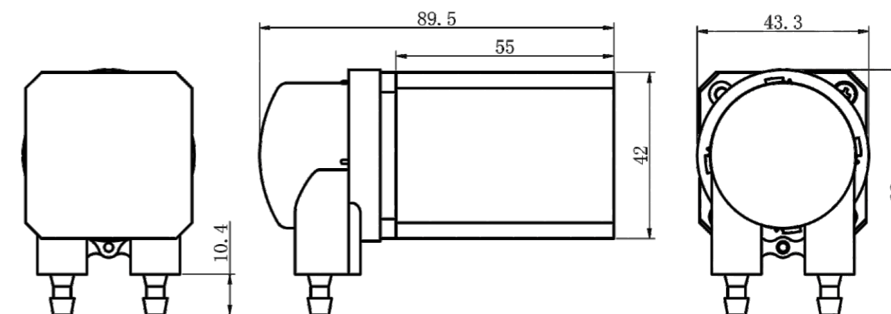
LFP101 Pump drawings:
