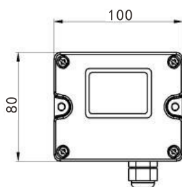
• LFH302 Duct Type Dimension
