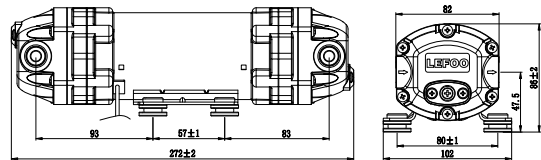
LFP2800J-FD (3/8" NPT)
