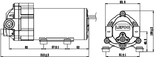
LFP2600W-A、LFP1600W-A (3/8" NPT)
