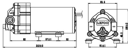
LFP1500W、LFP2500W (3/8 " NPT )
