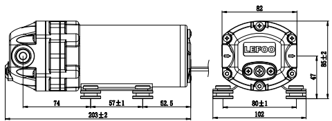
LFP1600J (3/8 " NPT )
