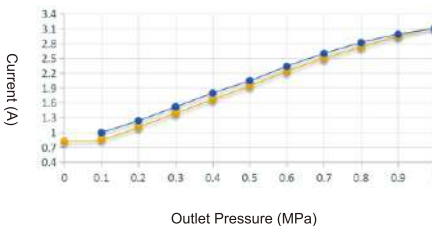
24V Normal Type - Line chart of pressure and current
