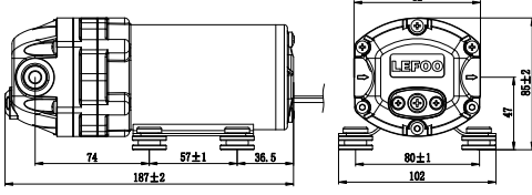
LFP1600JD (3/8 " NPT )
