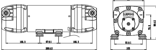
LFP21000W-FD (3/8" SIDE FEMALE QUICK CONNECTOR)
