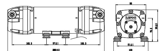
LFP21000W-FD1 (3/8" SIDE FEMALE QUICK CONNECTOR)
